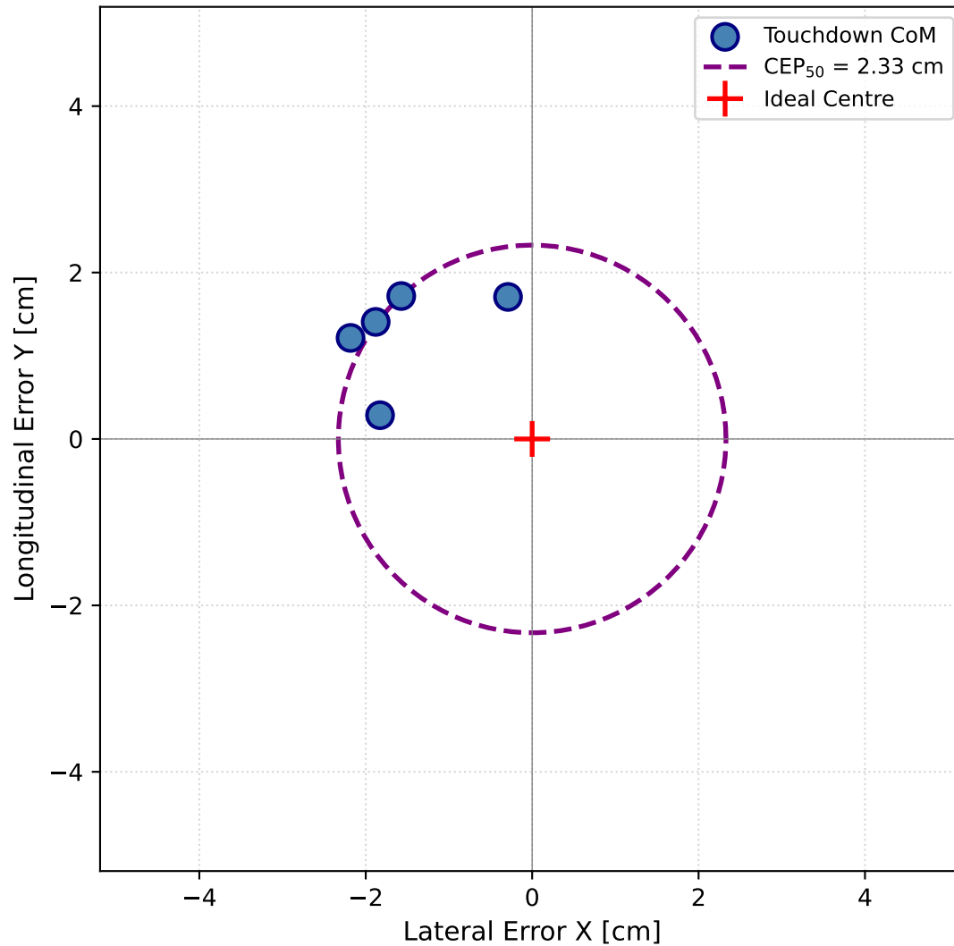
Touchdown Dispersion (CoM)
